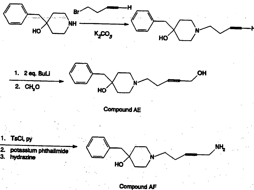
Scheme 12
